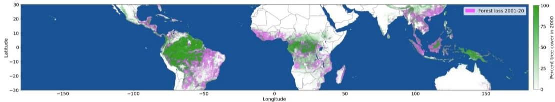
Tree cover in 2000 and Forest loss 2001-20
